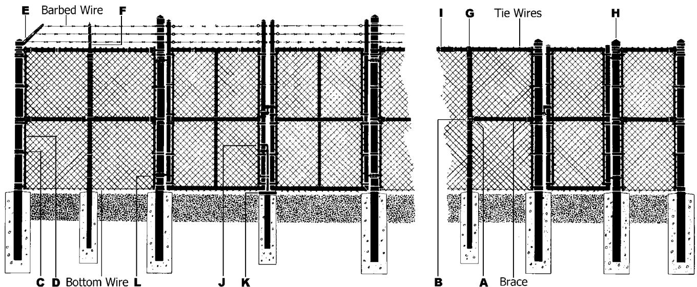
Double Gate – With 3 strands of barbed wire
